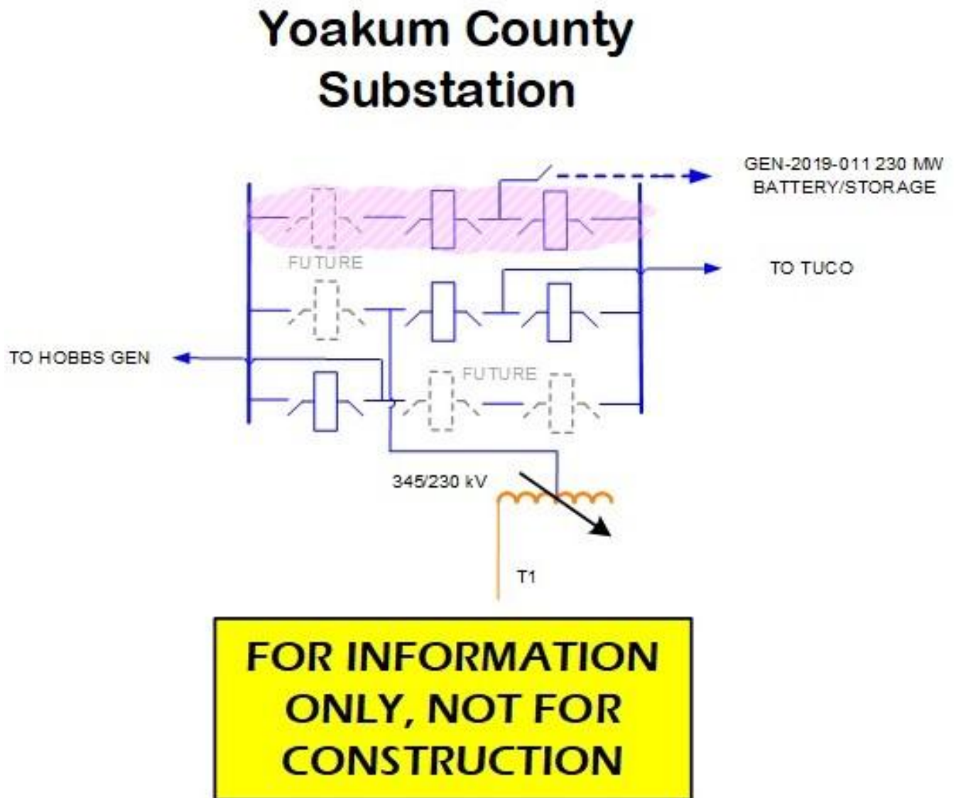
Figure 4 – Informational One-Line Drawing
